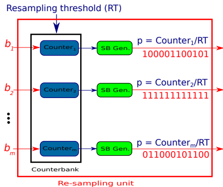
Fig. 6. Re-sampling unit.
