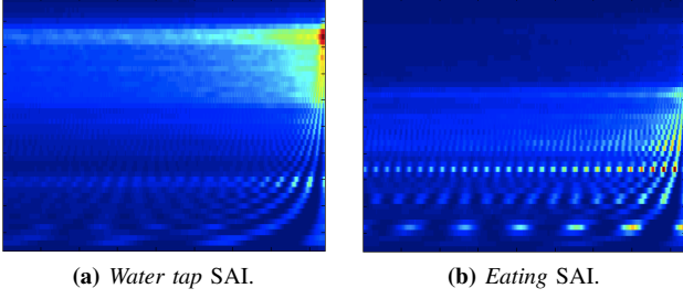
Fig. 3: Two examples of SAI in the time delay-frequency representation: (a) Running the tap and (b) Eating . The color encodes the intensity: the lighter the more intense. The time axis and the frequency axis are respectively on the abscissa and on the ordinate. Notice how the difference in timbre and resonance are emphasized in the frequency and time dimensions respectively.
