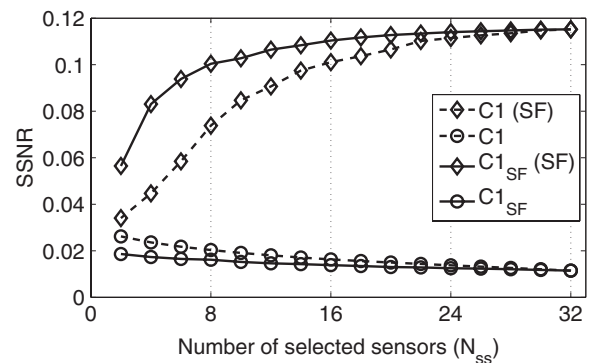
Figure 4. Evolution of the SSNR with and without SF in relation to the number of selected sensors ( N_{ss} ) for the selection methods C1 and C1 SF .
