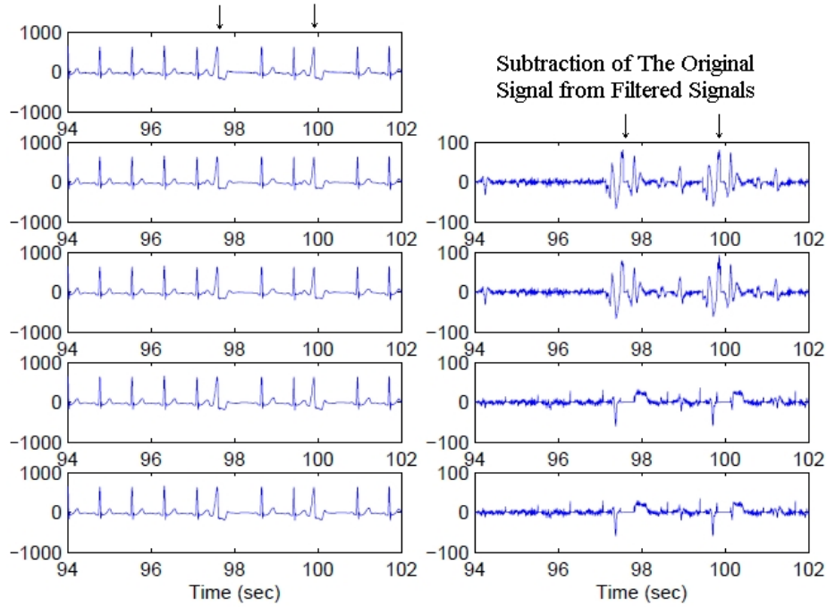
Figure 2: Illustration of proposed method on real data. Left, Up to Down: Original record 116 of the MIT-BIH Arrhythmia Database, 'strict' linear, 'flexible' linear, DTW, 'flexible' DTW outputs. Right, Up to Down: Subtraction of the original ECG from 'strict' linear, 'flexible' linear, DTW, 'flexible' DTW outputs.
