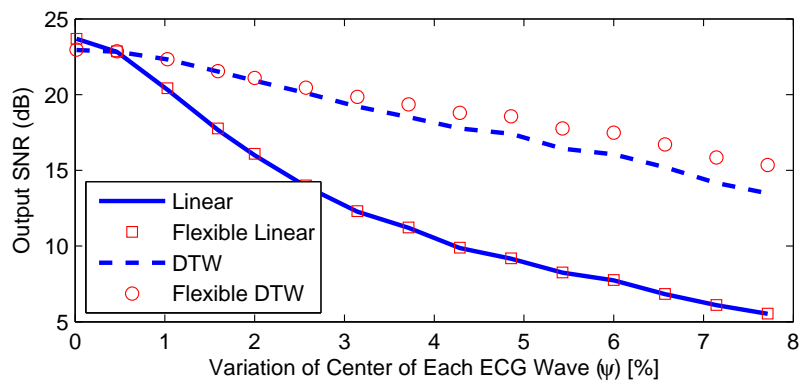
Figure 3: Mean value of EKF output SNR for different range of \psi variations
