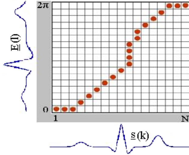
Figure 1: A typical example of DTW method for finding optimal match between reference ECG beat and current ECG beat.
