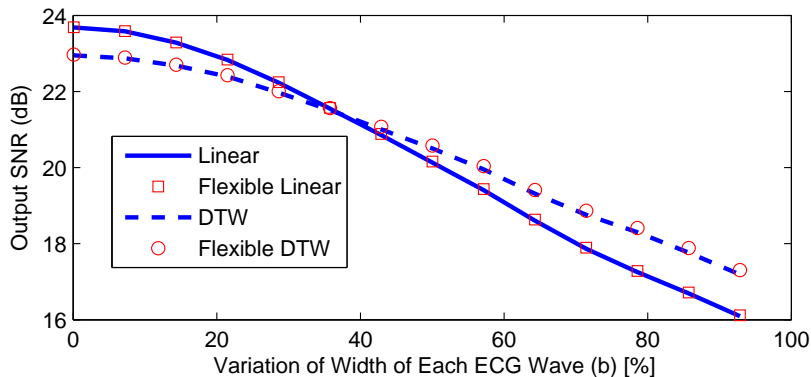
Figure 4: Mean value of EKF output SNR for different range of b variations
