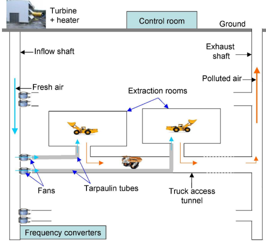
Figure 1. Airflows in an underground mine.
