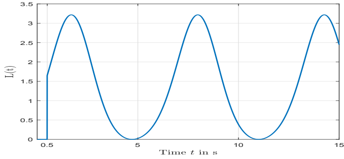
Figure 1. Calculated observer gain L(t)
