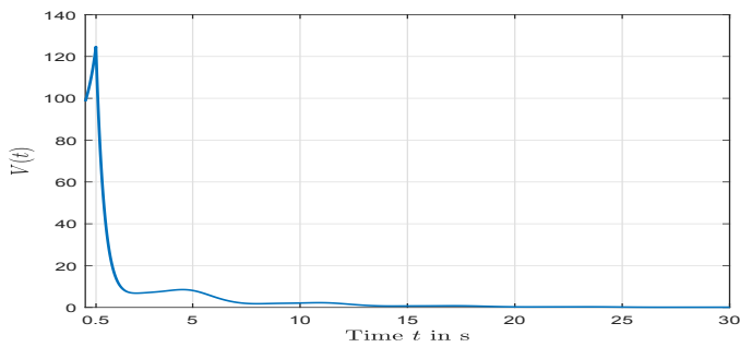
Figure 4. Lyapunov function V(t)
