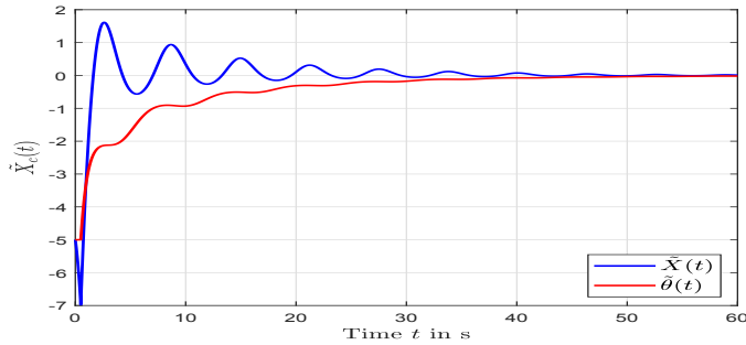
Figure 3. Estimation error of the ODE states \tilde{X}(t) and \tilde{\theta}(t)
